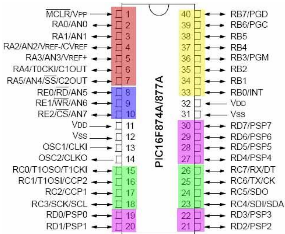
Figure 7 PIC 16F877A Pin Configuration
