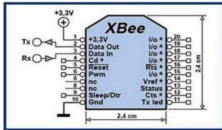
Figure 6 Zigbee pin configuration
