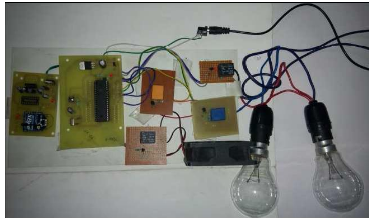
Figure 2 Receiver Module
