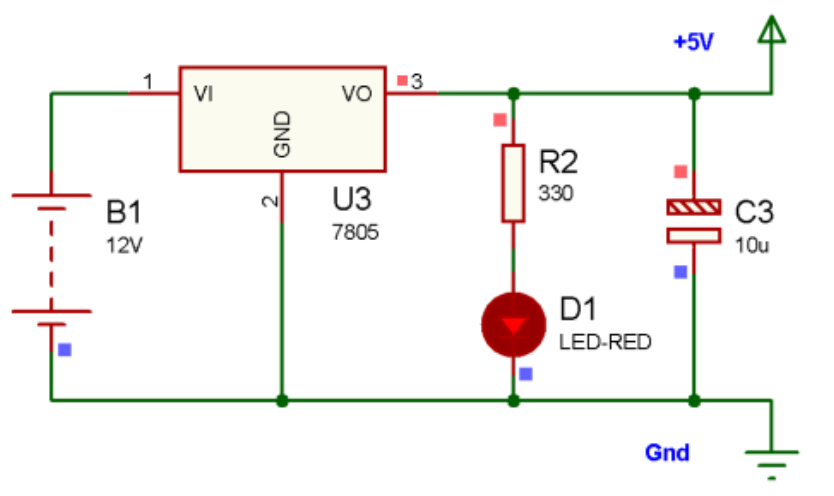
Figure 9 Battery operated +5V power supply
