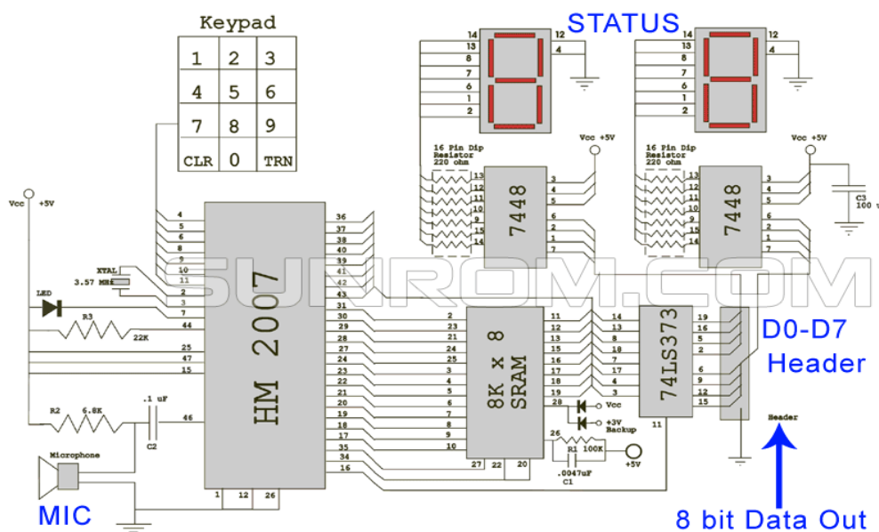
Figure 3 Functional Pin Description of HM 2007
