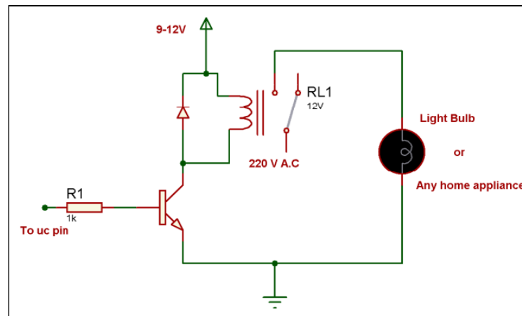
Figure 10 Relays switch board interfacing with the microcontroller
