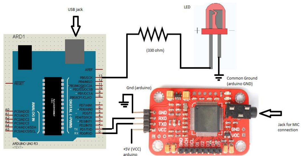
Figure 4 Schematic diagram
