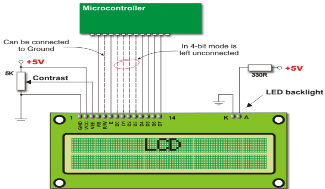
Figure 8 LCD Basic Connection
